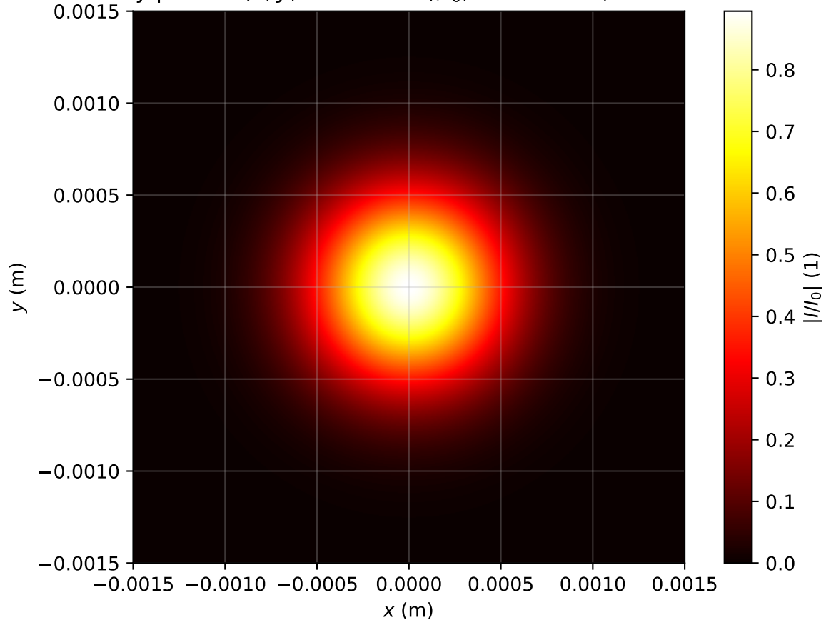
Intensity profile I(x, y, z = 0.796m)/I_0 , Pin=0.1Pcr, artificial time
